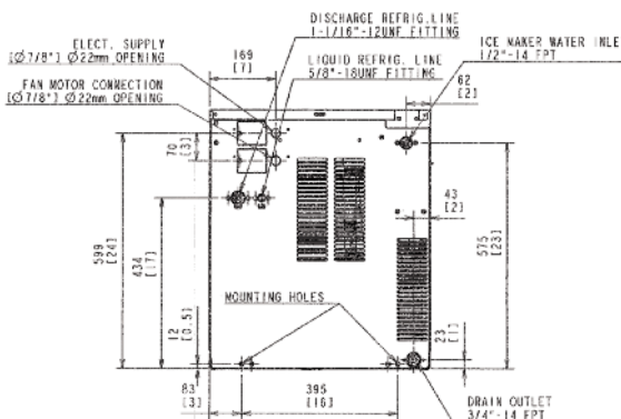
REMOTE AIR-COOLED UNIT
