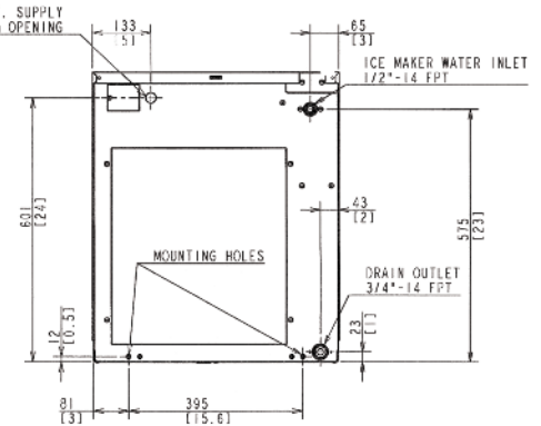
AIR-COOLED UNIT
