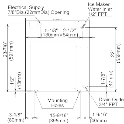
AIR-COOLED UNIT
