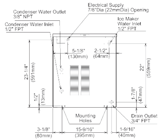
WATER-COOLED UNIT
