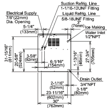
F-200I / BACK VIEW
