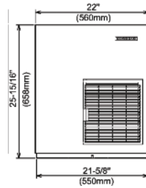
F-100I / FRONT VIEW
