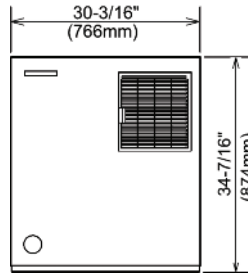
F-200I / FRONT VIEW
