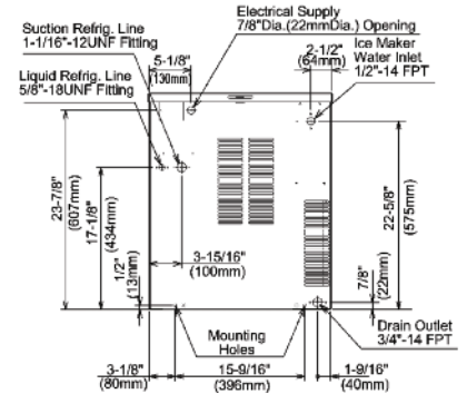
F-100I / BACK VIEW
