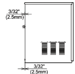
F-200I / RIGHT SIDE VIEW
